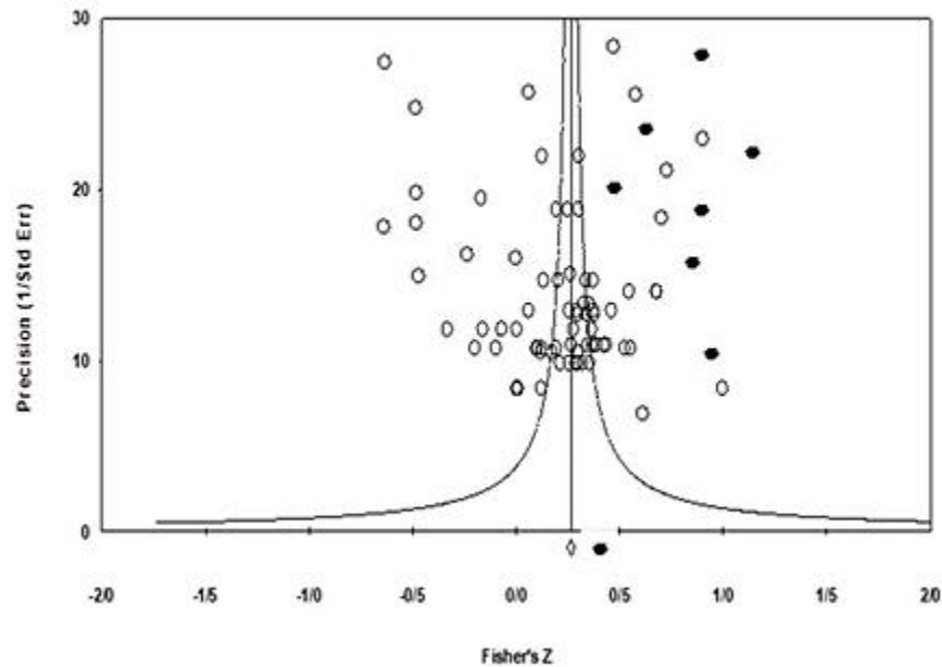
Figure 5: Adjusted funnel diagram using accuracy indicators
