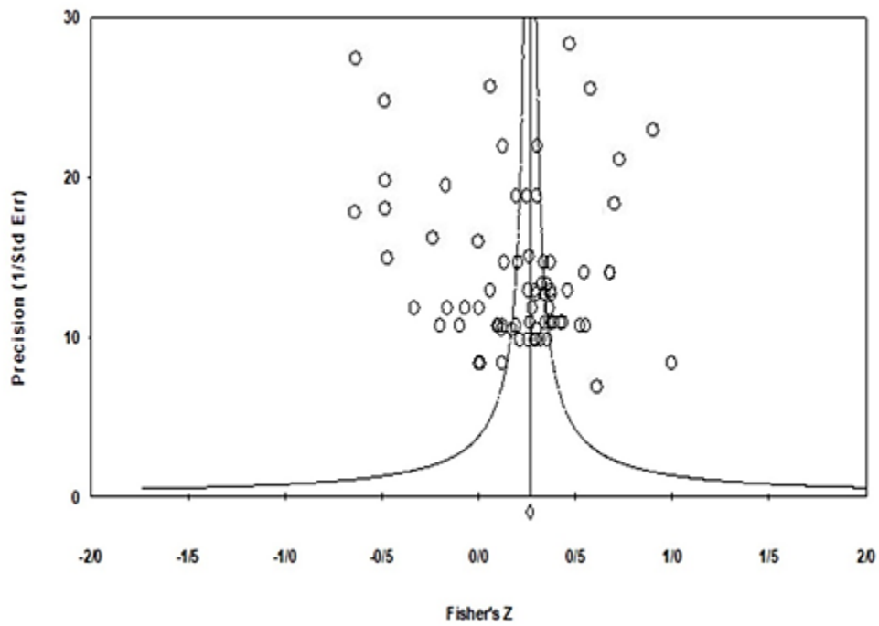
Figure 3: Funnel plot using indicators of accuracy
