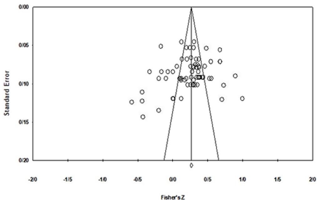
Figure 2: Funnel plot using standard error indicators in studies pertaining to the research question
