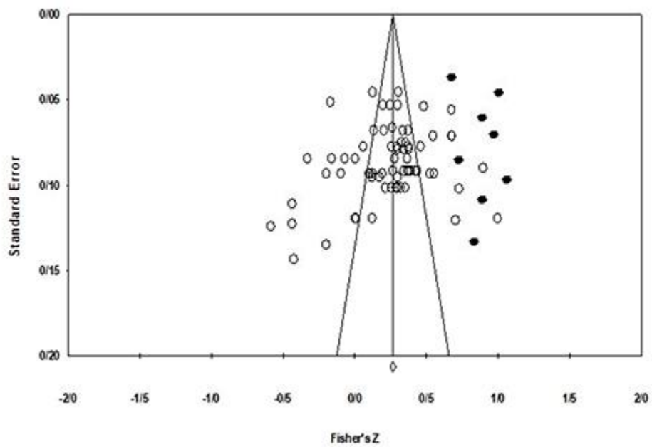
Figure 4: Adjusted funnel plot using standard error indicators related to the research question
